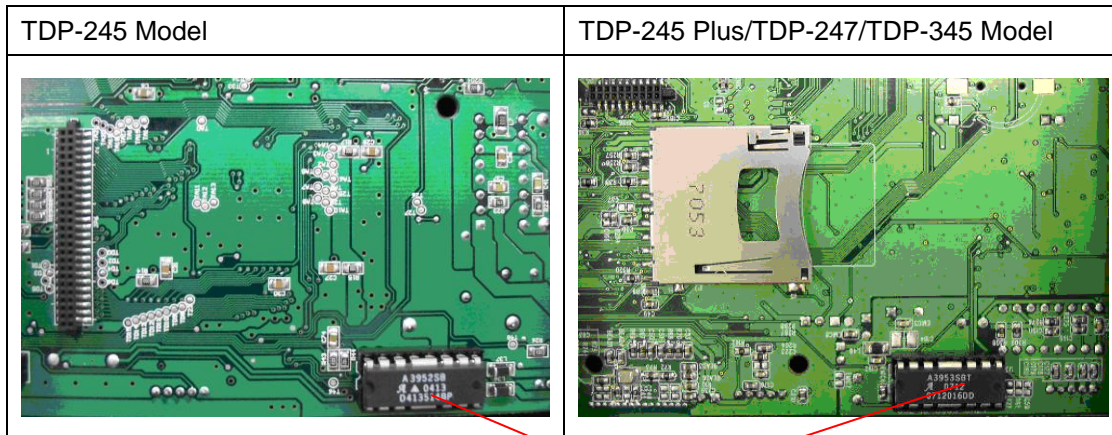
Cutter Driver IC
